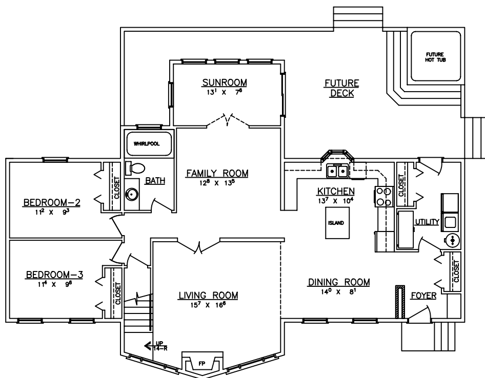
MAIN FLOOR AREA = 1422 S.F.
