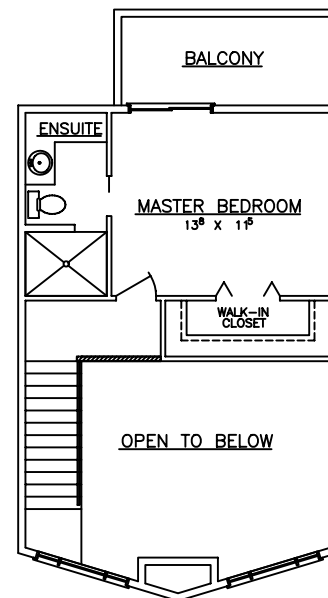
SECOND FLOOR AREA = 320 S.F.
